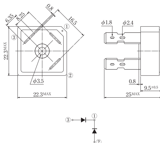
Fig.76 Package: D30VC
