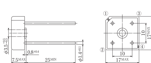
Fig.62 Package: S4VB
