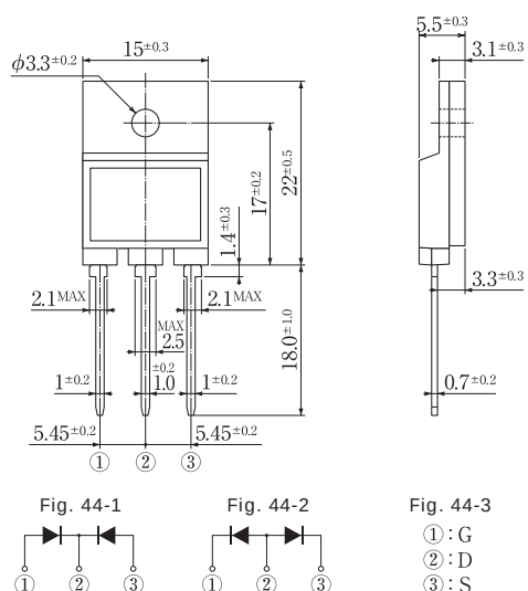
Fig.44 Package: ITO-3P
