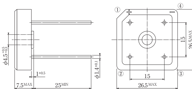
Fig.70 Package: S15WB
