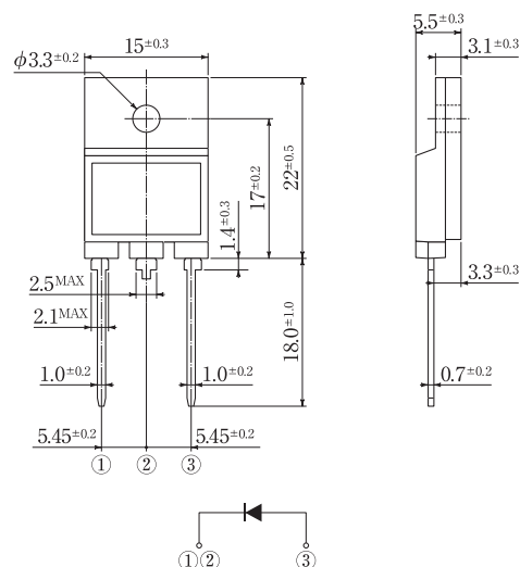
Fig.43 Package: ITO-3P
