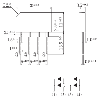
Fig.56 Package: 2S
