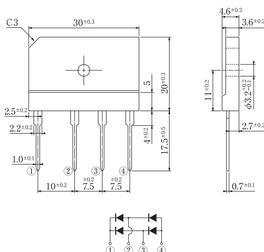
Fig.58 Package: 5S
