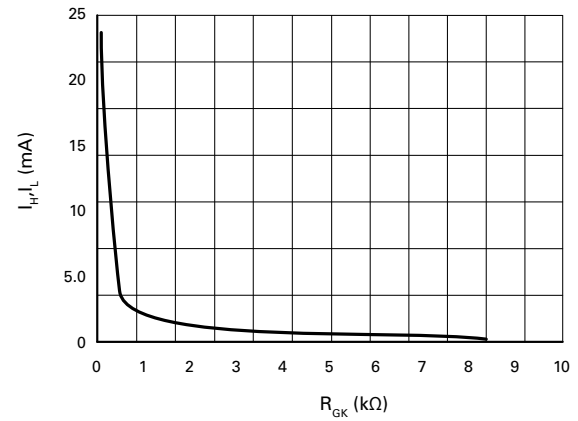
Figure 9. Holding and Latching Current vs. R_{GK}
