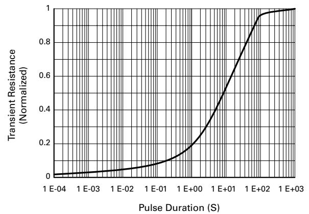
Figure 4. Thermal Response
