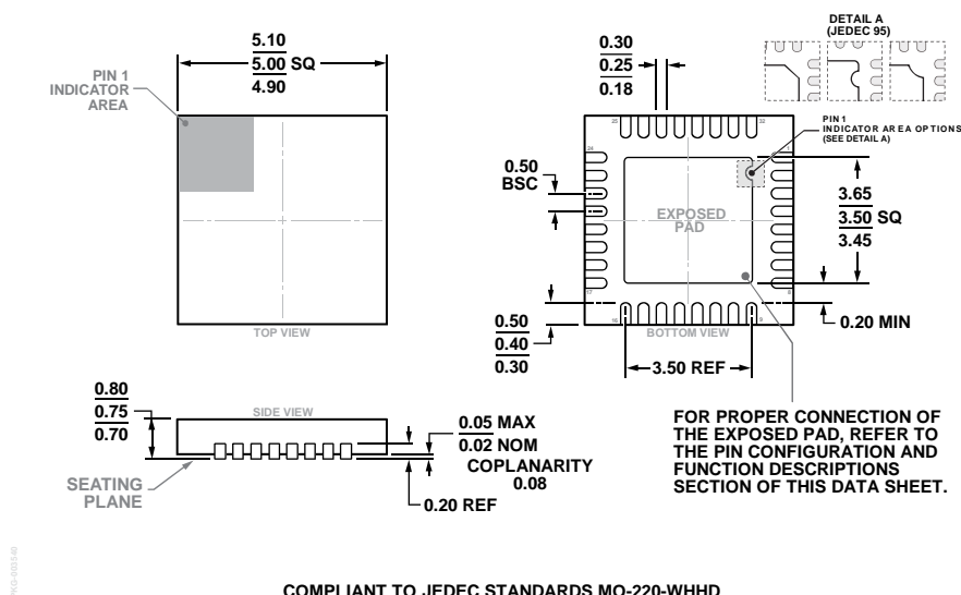
COMPLIANT TO JEDEC STANDARDS MO-220-WHHD Figure 55. 32-Lead Lead Frame Chip Scale Package [LFCSP] 5 mm x 5 mm Body and 0.75 mm Package Height (CP-32-11) Dimensions shown in millimeters
