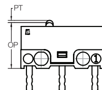
OP FROM BASE (FOR TYPE 20 & 30 TERMINAL)
