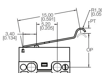
TYPE H SIMULATED ROLLER LEVER (15,0 mm; R1,3)
