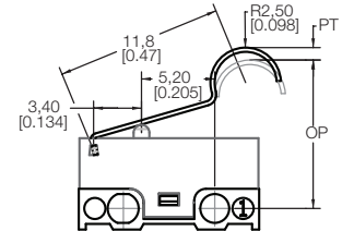
TYPE E SIMULATED ROLLER LEVER (11,8 mm; R2,5)
