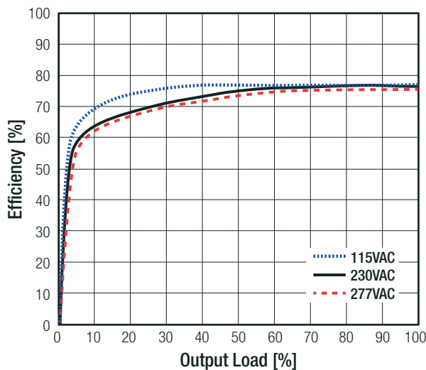
RAC04-05SK/277
