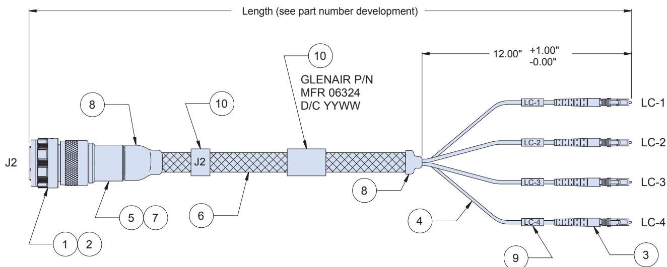
Connection Diagram
