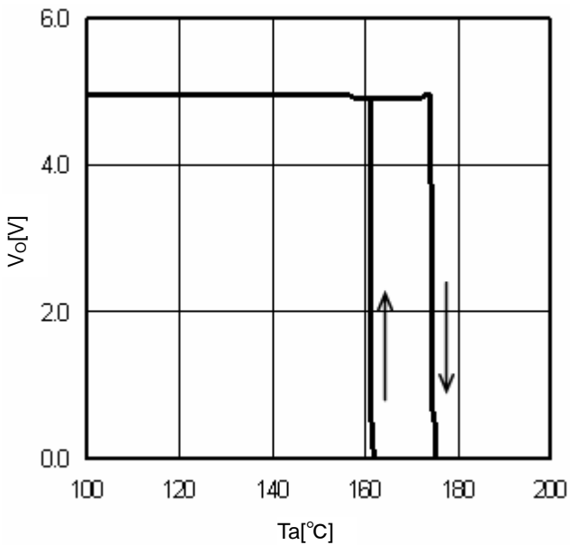
Fig.15 TSD ( I_o=0mA )
