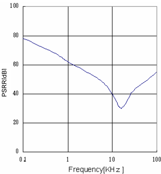
Fig.20 PSRR ( I_o=0mA )
