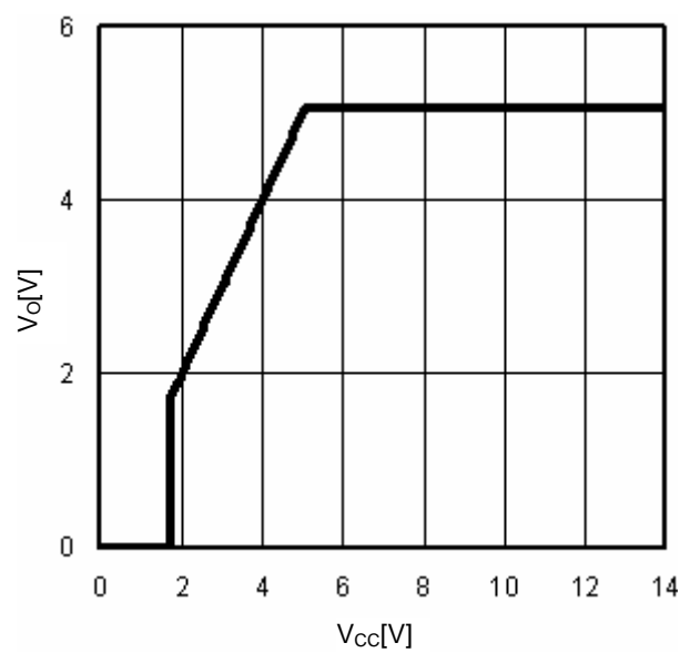
Fig.14 V_{cc}-V_o ( I_o=0mA )
