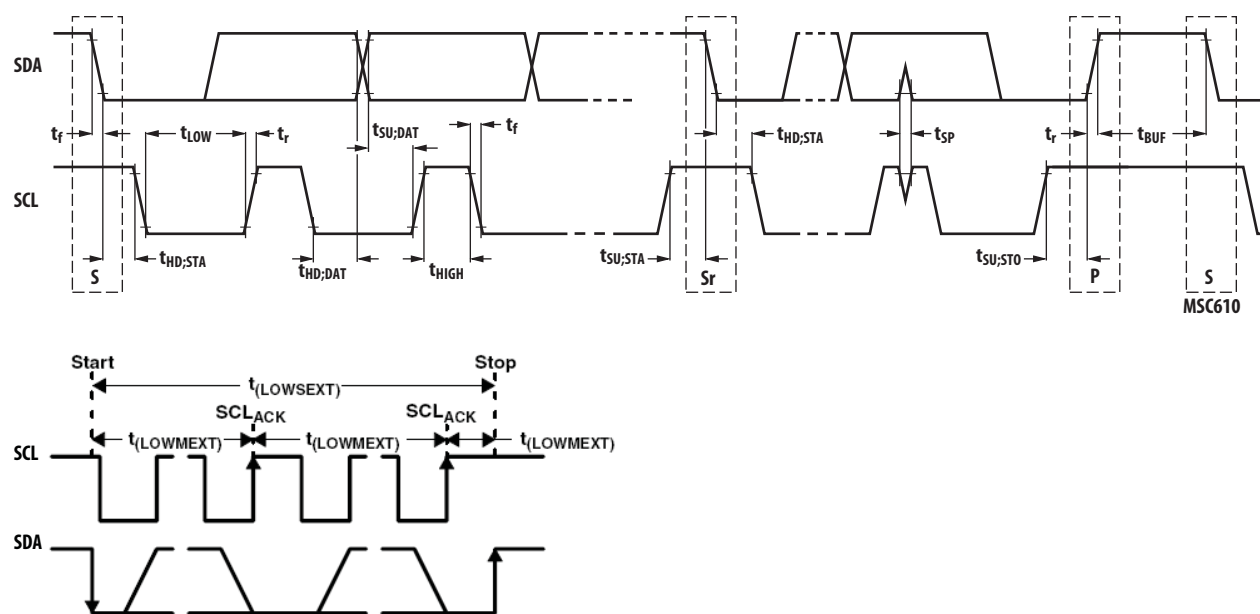
Figure 1. I 2 C Bus Timing Diagram
