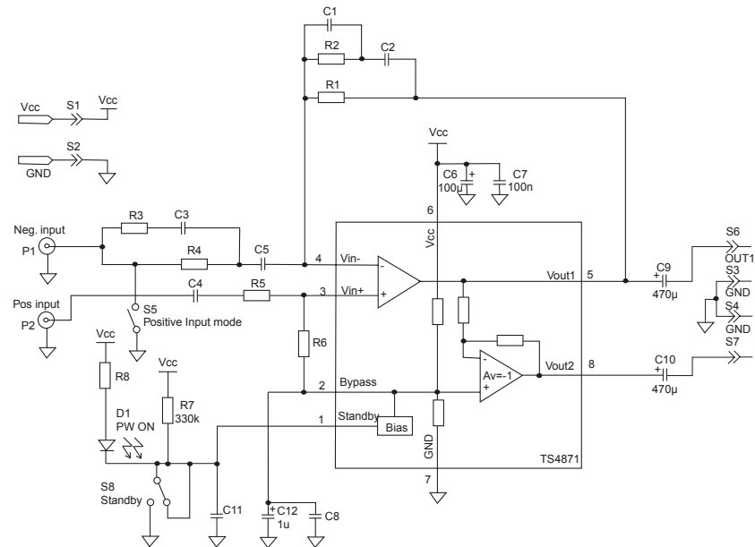
Figure 82. Demoboard schematic
