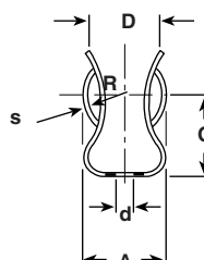
Figure 2: Spring clip
