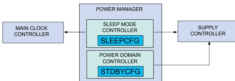
Figure 20-1. PM Block Diagram
