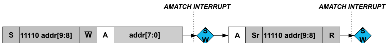
Figure 34-11. 10-bit Addressing
