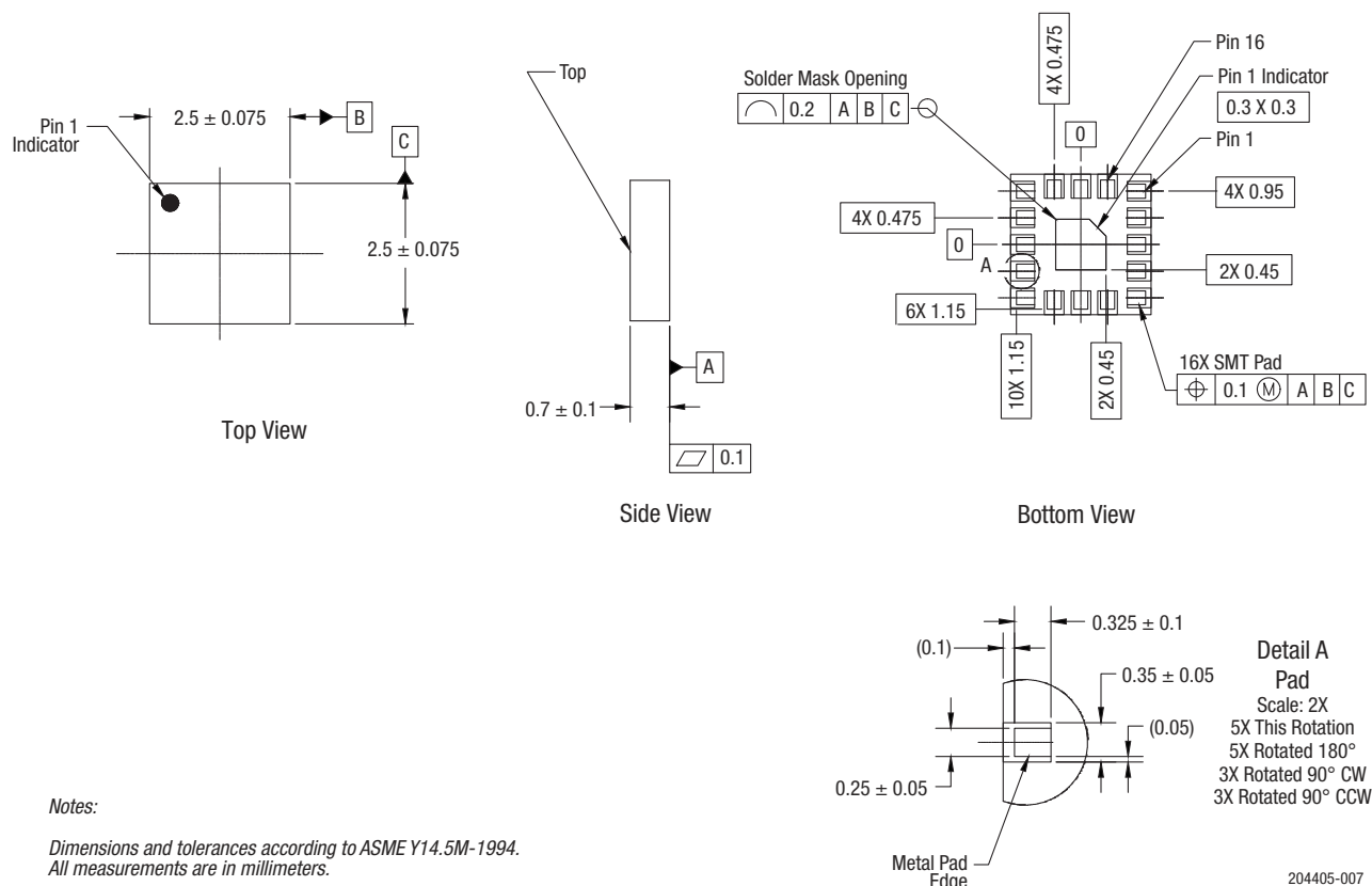
Figure 7. SKY65933-11 Package Dimensions
