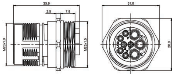
Receptacle, straight, M25 Checkmate™
