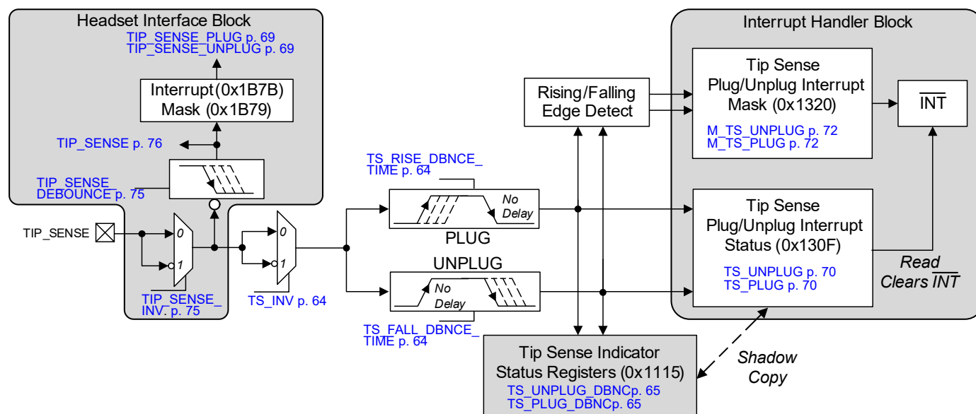
Figure 4-24. Tip-Sense Controls
