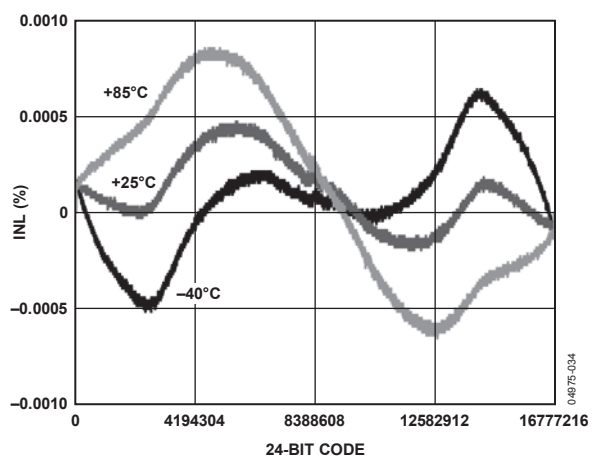
Figure 31. 24-Bit INL, Normal Mode
