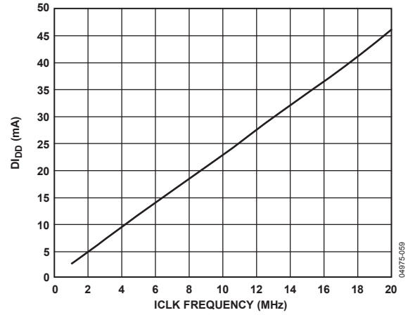
Figure 38. Decimate \times 32, D_{IDD} vs. ICLK Frequency ( V_{DD} = 2.5\text{ V} )
