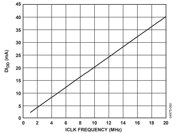
Figure 39. Decimate \times 256, D_{IDD} vs. ICLK Frequency ( V_{DD} = 2.5\text{ V} )
