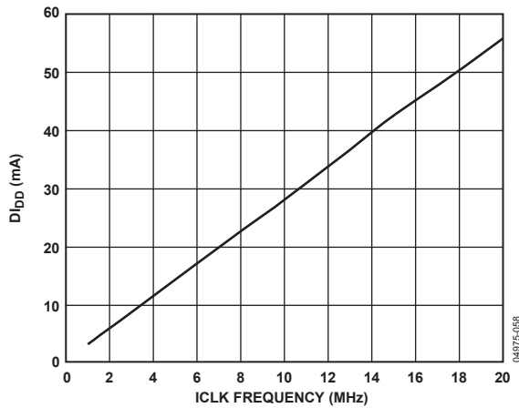
Figure 37. Decimate \times 8, D_{IDD} vs. ICLK Frequency ( V_{DD} = 2.5\text{ V} )
