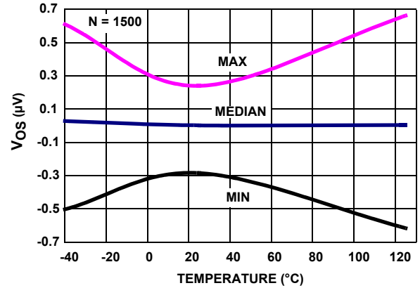
FIGURE 20. EL8172 V_{OS} vs TEMPERATURE, V_+, V_- = \pm 2.5V, V_{IN} = 0V
