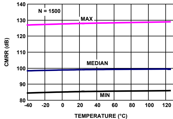
FIGURE 24. EL8172 CMRR vs TEMPERATURE, V_{CM} = +2.5V TO -2.5V , V_+ , V_- = \pm 2.5V
