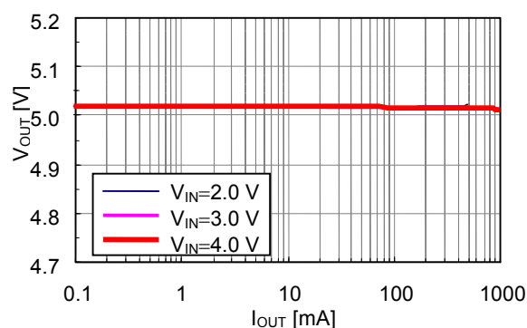
(b) Output current ( I_{OUT} ) vs. Output voltage ( V_{OUT} )
