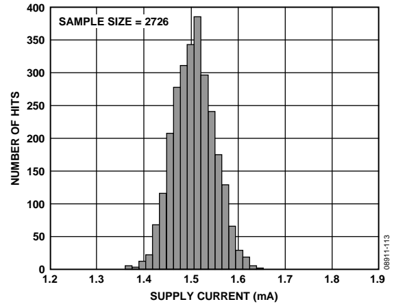
Figure 13. Supply Current
