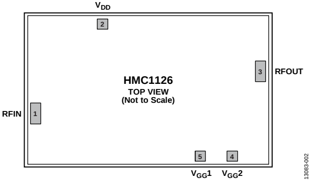
Figure 2. Pad Configuration
