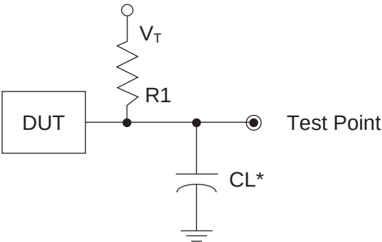
Figure 3-21. Output Test Load, LVTTTL and LVCMOS Standards
