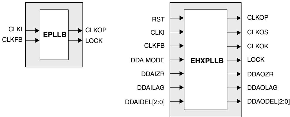
Figure 2-12. PLL Primitive
