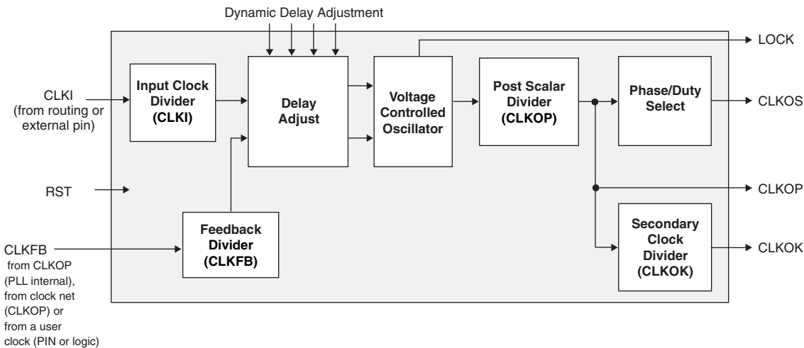
Figure 2-11. PLL Diagram
