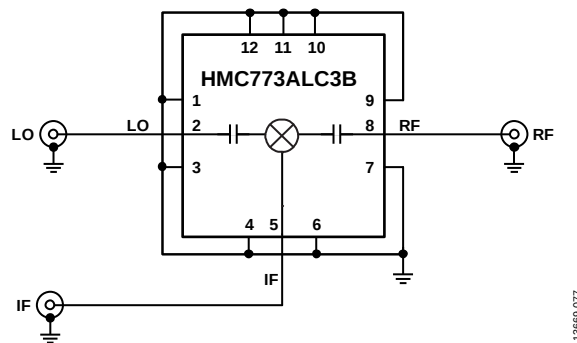
Figure 77. Typical Application Circuit
