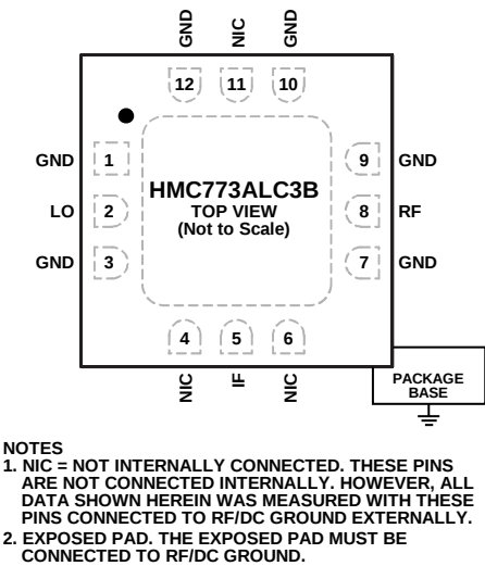
Figure 2. Pin Configuration
