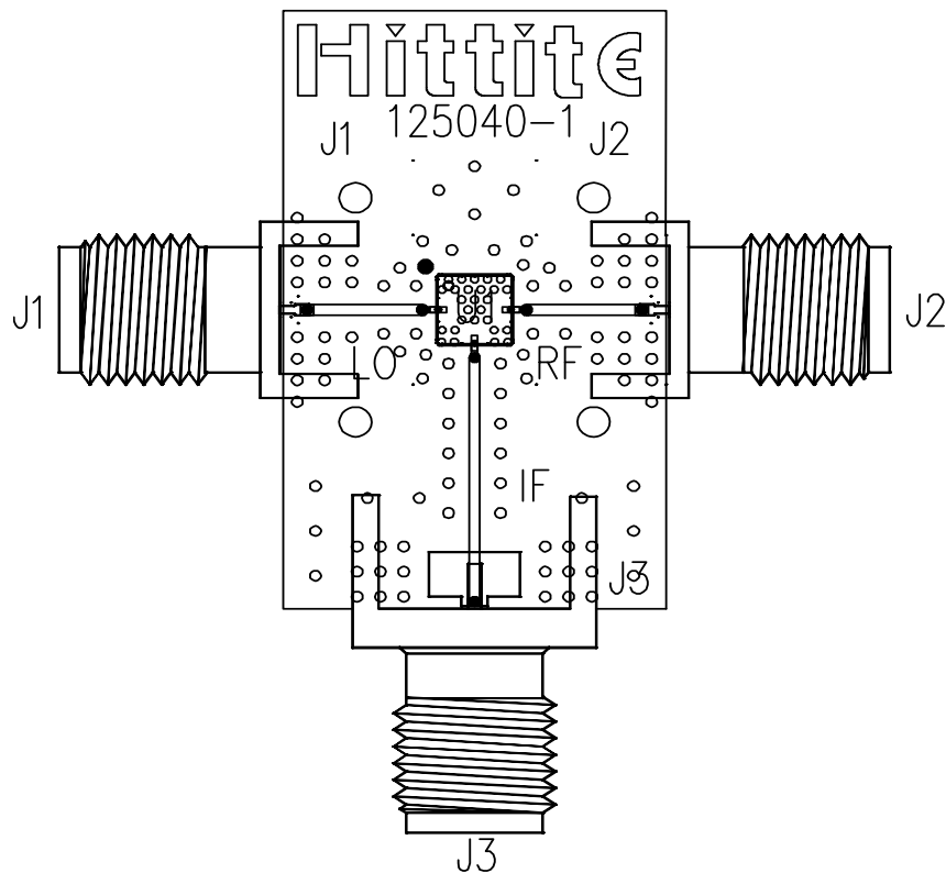
Figure 78. Evaluation PCB
