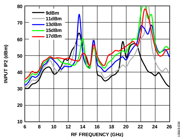
Figure 38. Input IP2 vs. RF Frequency at Various LO Drives
