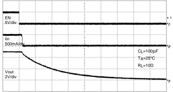
Turn-Off Delay and Fall Time
