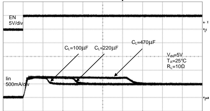
Inrush Current with Different Load Capacitance
