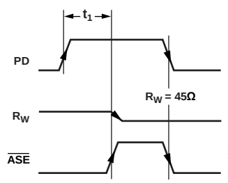
Figure 6. End Scale Indication Timing
