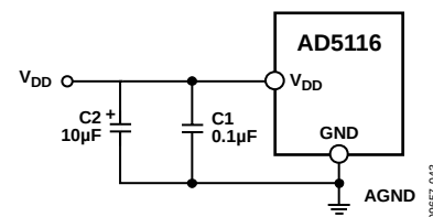
Figure 45. Power Supply Bypassing
