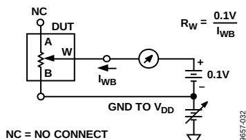
Figure 34. Wiper Resistance
