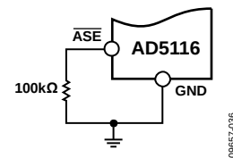
Figure 38. Automatic Store Enables
