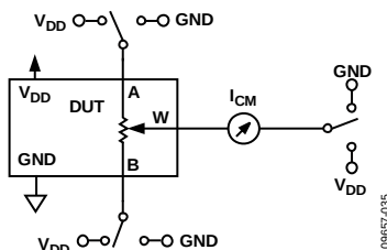
Figure 37. Common-Mode Leakage Current
