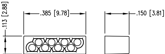
MANAGEMENT BAR P/N 370808M2-MB
