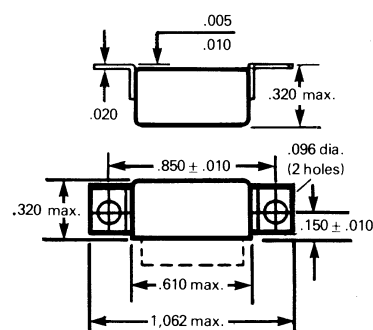
Side Bracket
