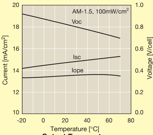
Output Temperature Dependency Characteristics
