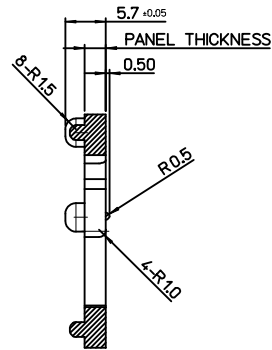
VIEW "X"
