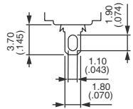
Solder lugs
