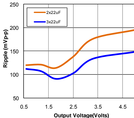
Fig-1: Input ripple voltage for various output voltages with 2x22uF or 3x22uF ceramic capacitors at the input (12A load). Input voltage is 12V.
