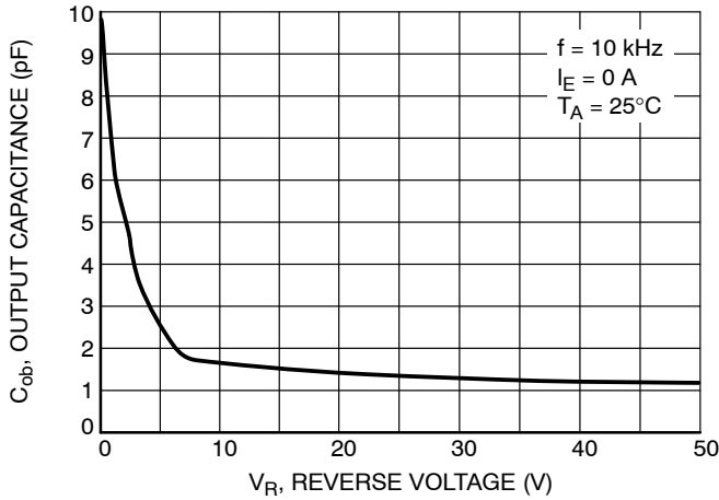
Figure 4. Output Capacitance
