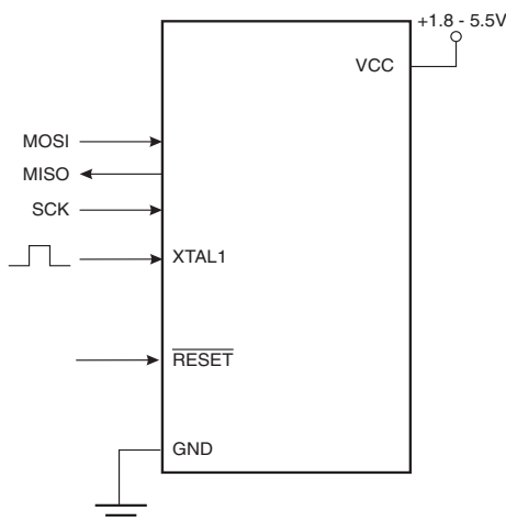
Figure 78. Serial Programming and Verify
