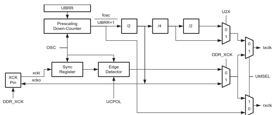
Figure 54. Clock Generation Logic, Block Diagram
