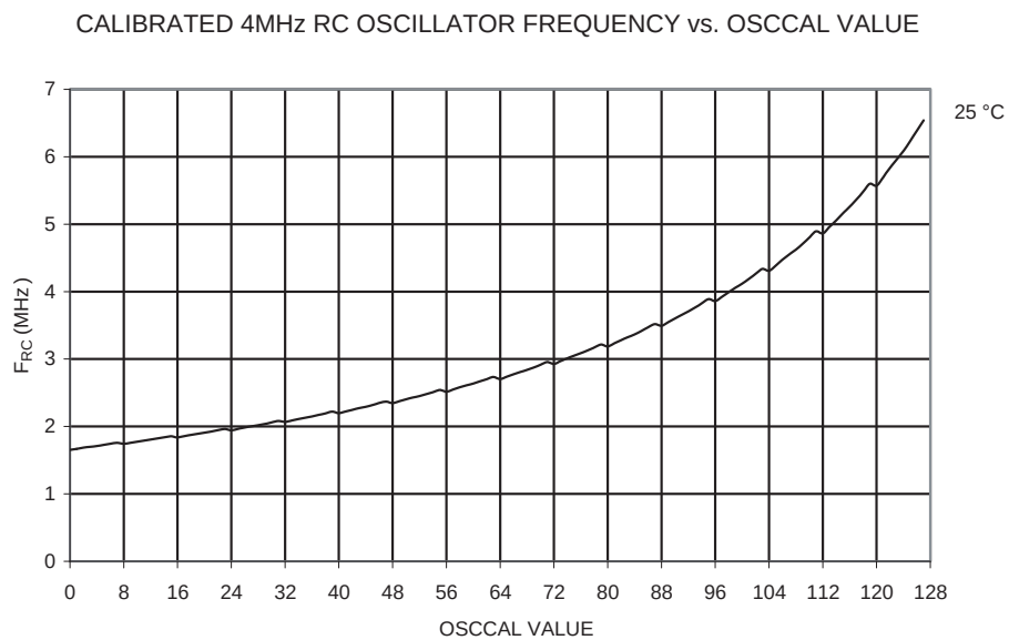
Figure 136. Calibrated 4 MHz RC Oscillator Frequency vs. Oscscal Value
