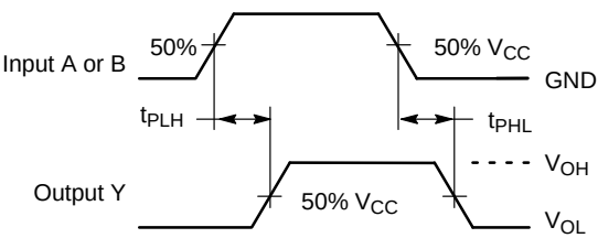
Figure 2. Switching Waveforms
