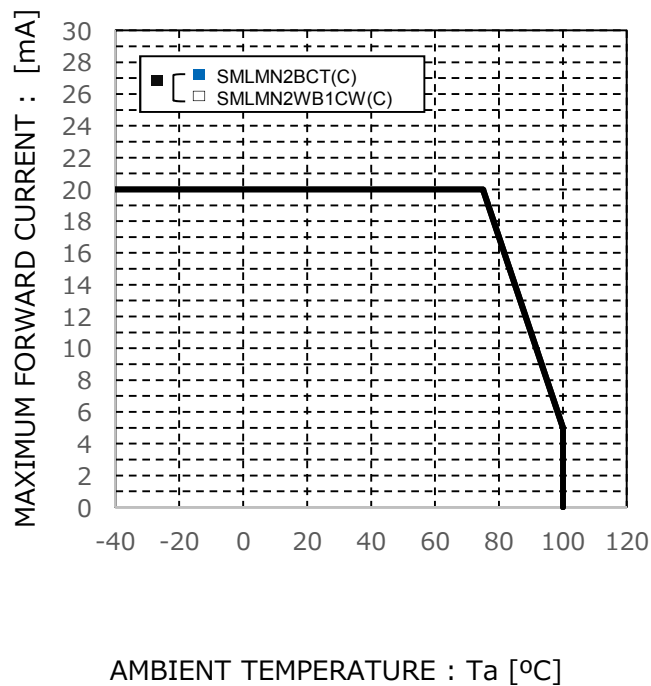
Fig.4 Derating
