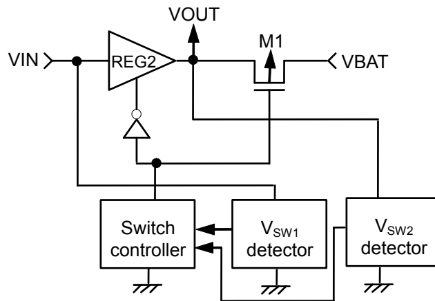
Figure 8 Switch Unit
