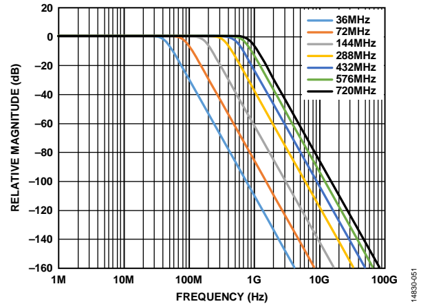
Figure 66. Ideal Fourth-Order Butterworth Magnitude Response for All 1 dB Bandwidths Programmed
