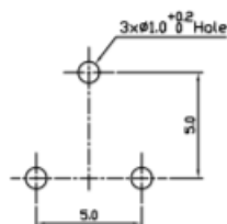
PCB MOUNTING PATTERN
