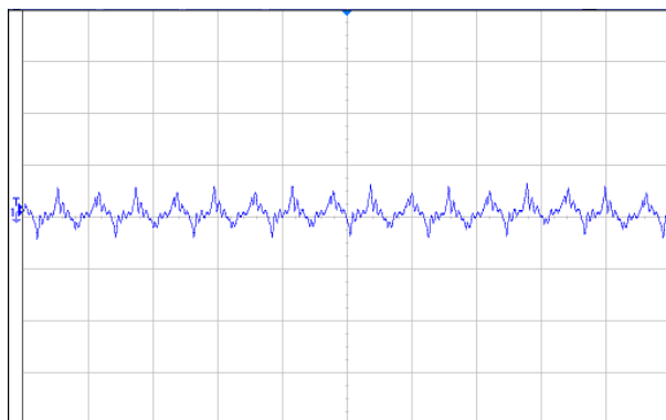
Figure 2 Output ripple & noise (5 \mu\text{s/div} , 50mV/div), see Figure 15 for test configuration
