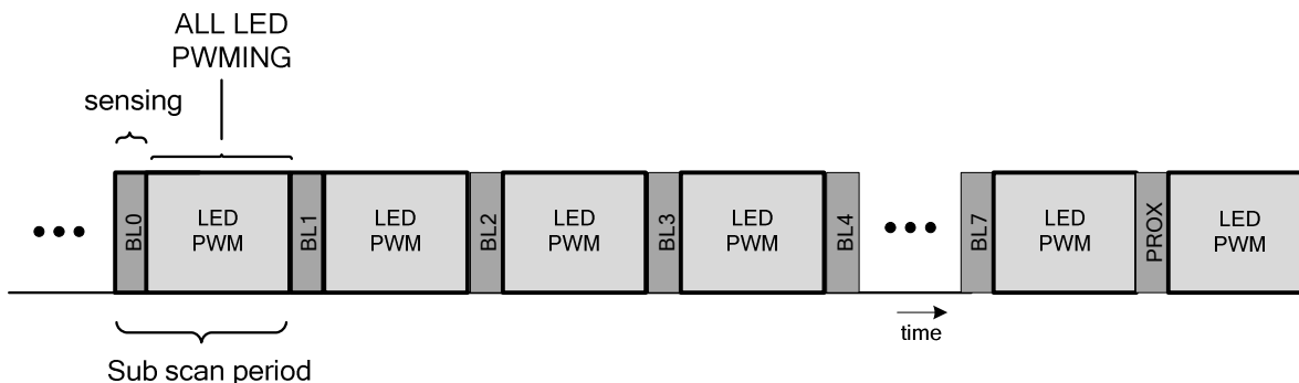
Figure 7 CapSense Scan Frame SX9510/11
