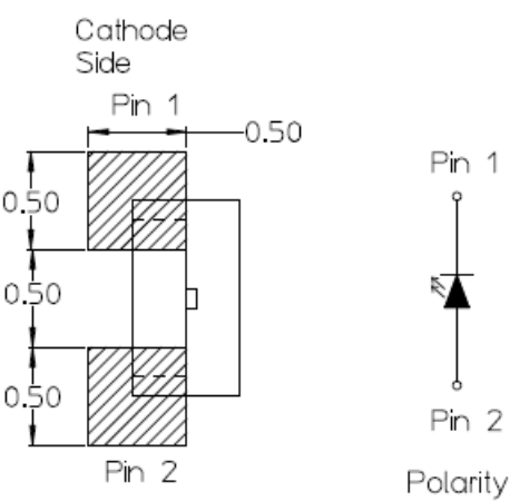
Figure 11: Recommended Solder Pad (Units: mm)
