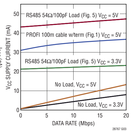
V_{CC} Supply Current vs Data Rate
