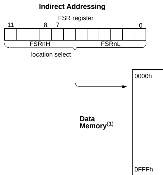
FIGURE 4-6: INDIRECT ADDRESSING
