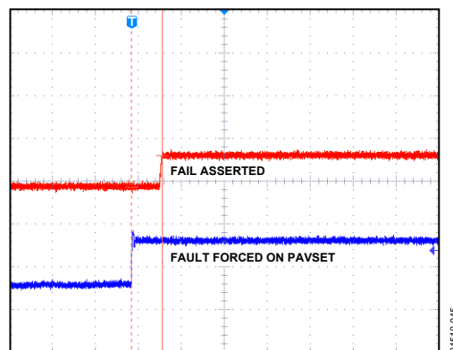
Figure 16. FAIL Assert Time, 1 µs/DIV
