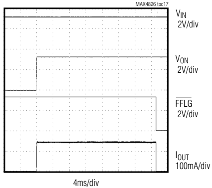
FFLG-BLANKING RESPONSE
