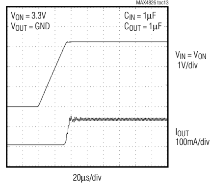
CURRENT-LIMIT RESPONSE
