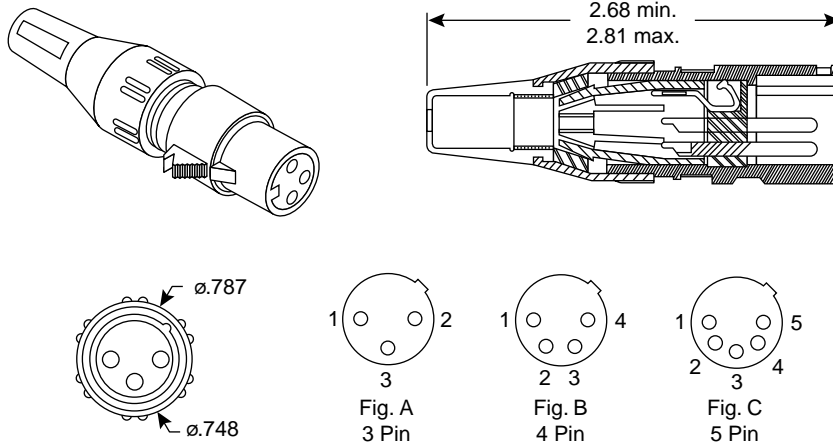
Dimensions (In.)
