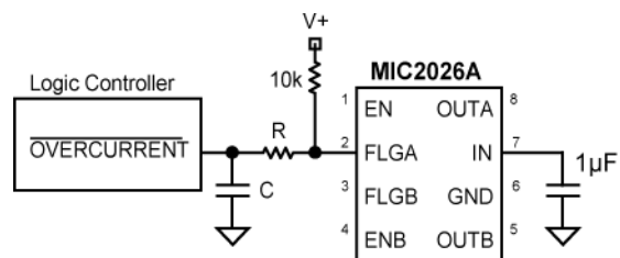
Figure 4. Transient Filter
